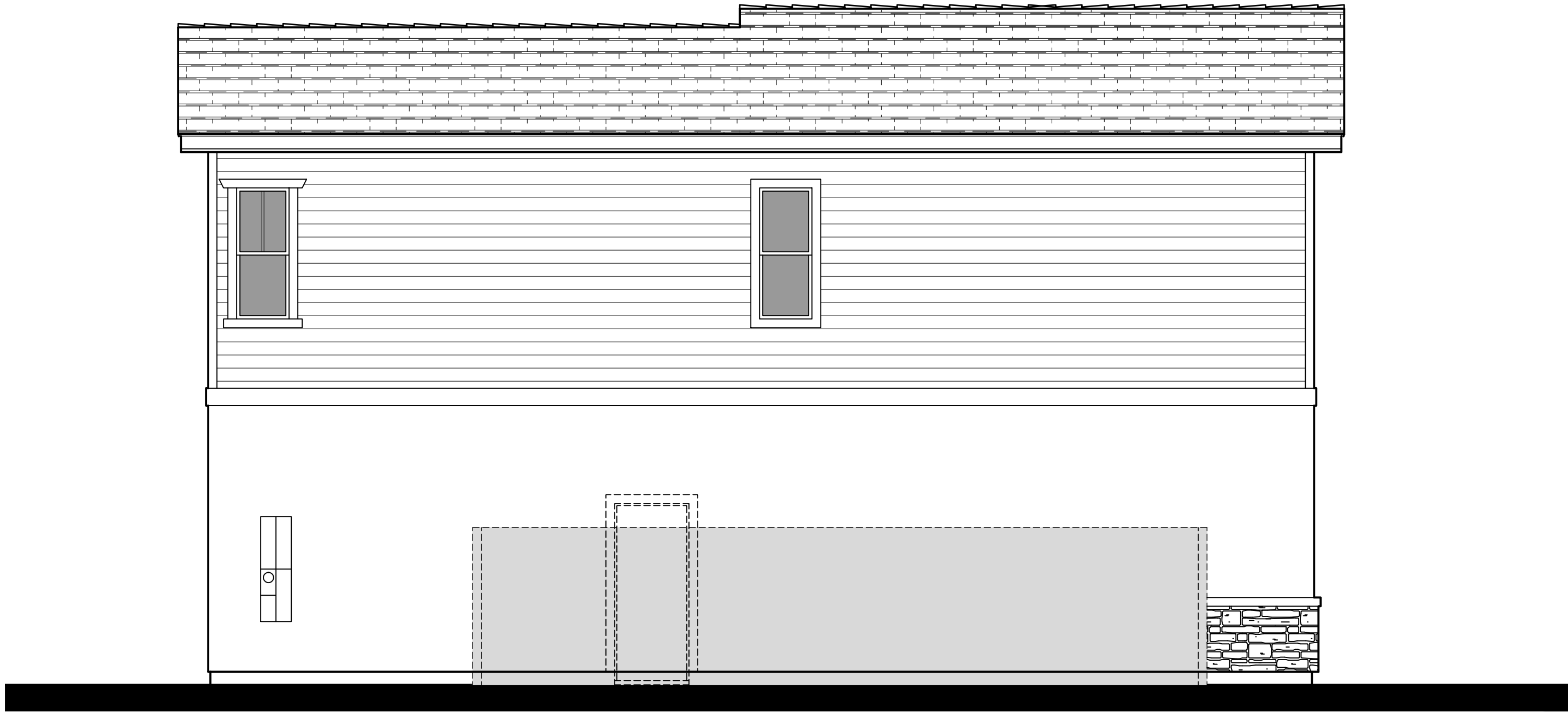
Left Elevation
