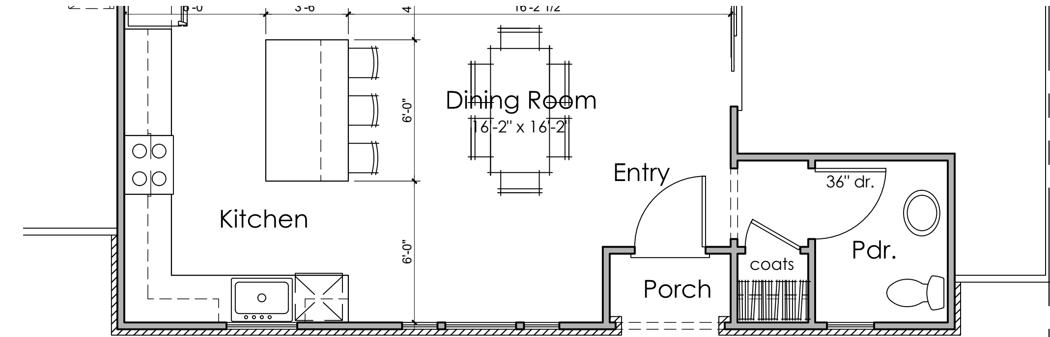
First Floor 811 SQ. FT.
