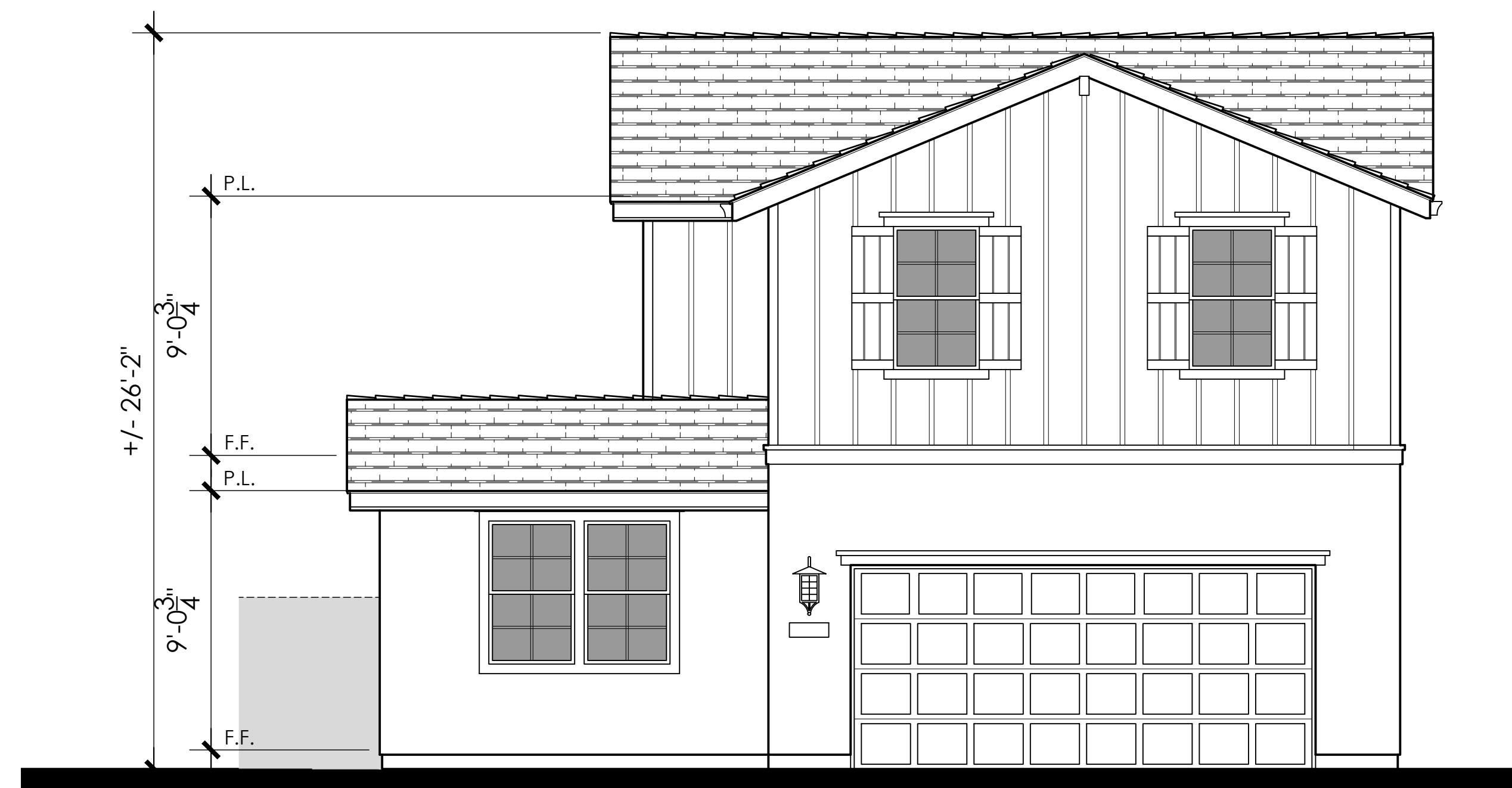
Rear Elevation
